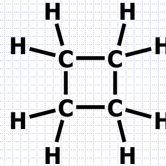
Cyclobutan
