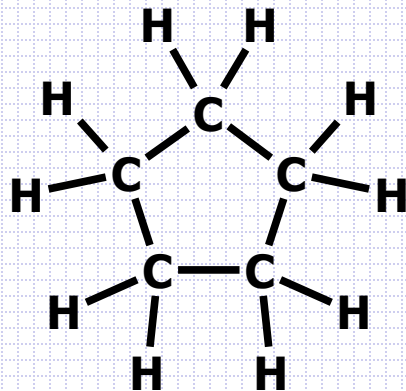
Cyclopentan
