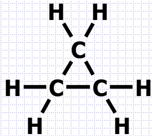
Cyclopropan
